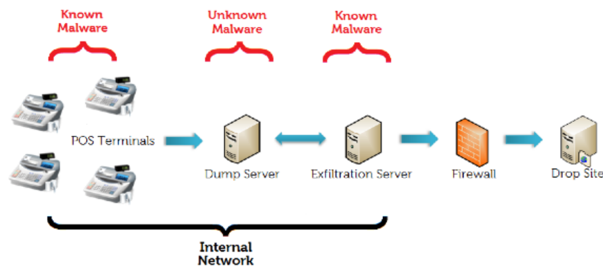
Figure 2 - Diagram of Data Exfiltration
